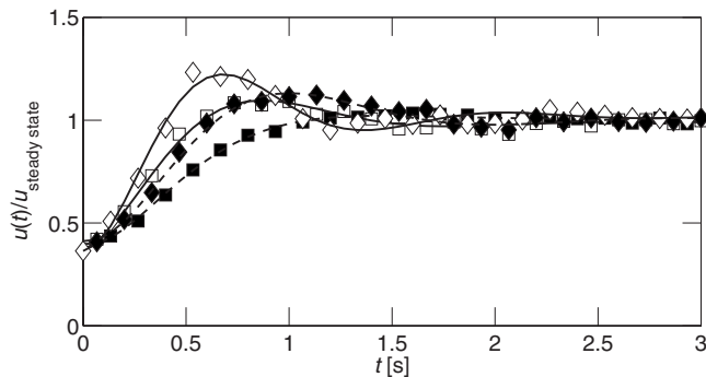
FIG. 9. Streamwise velocity (relative to final velocity) at the free surface as a function of time following a step increase in the rotational speed at t=0 . ( \square ) d=1 mm particles and ( \diamond ) d=2 mm particles; open markers represent tumbler radius R=8.6 cm and filled markers represent R=13.9 cm. For clarity of the fitted step response, markers are only shown for half of the time steps.
